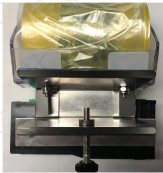
Mini T-Bracket Horizontal Assembly attaches directly to the bag holder.
