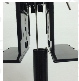
Assembly mounts into tube, using spring bar that hooks onto tube lip.
