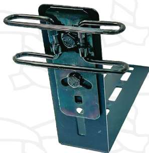
Part # 37152 UB Side Mount BRACKET ONLY
