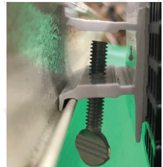
Tighten thumb screw to expand into price channel.
